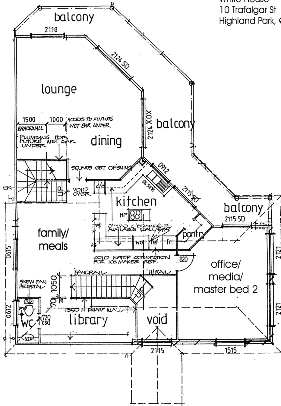
First Floor - Level 2
