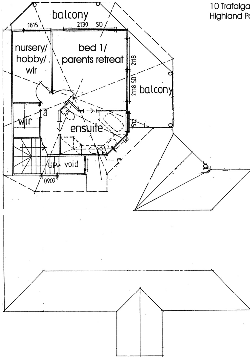
Second Floor - Level 3
